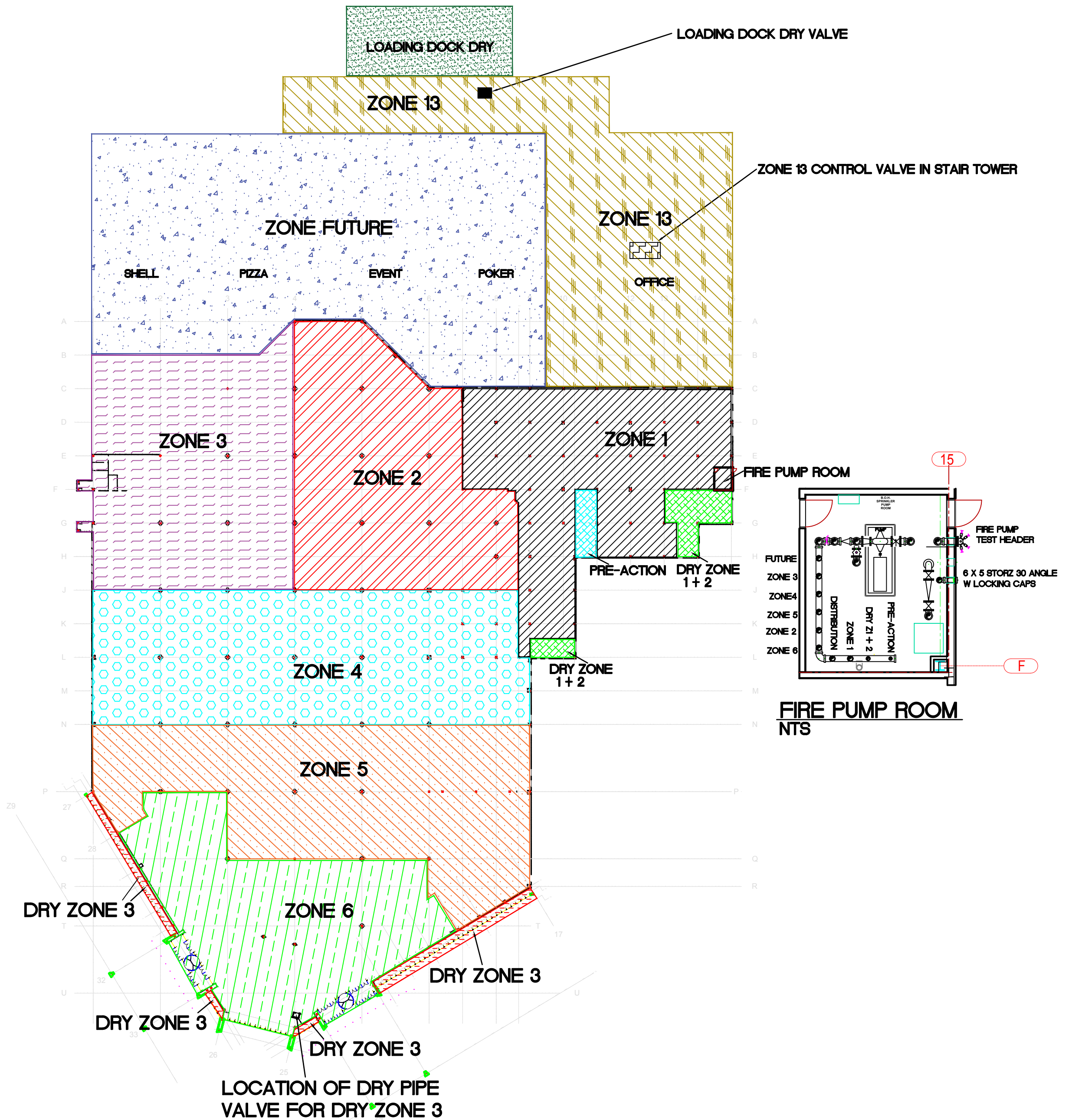
SPRINKLER ZONE PLAN NOT TO SCALE
